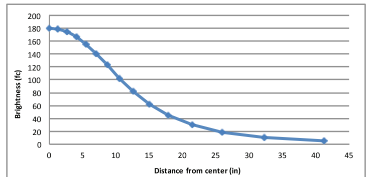
Photometrics for desk/floor lamps: Light source placed 15" away from work surface
