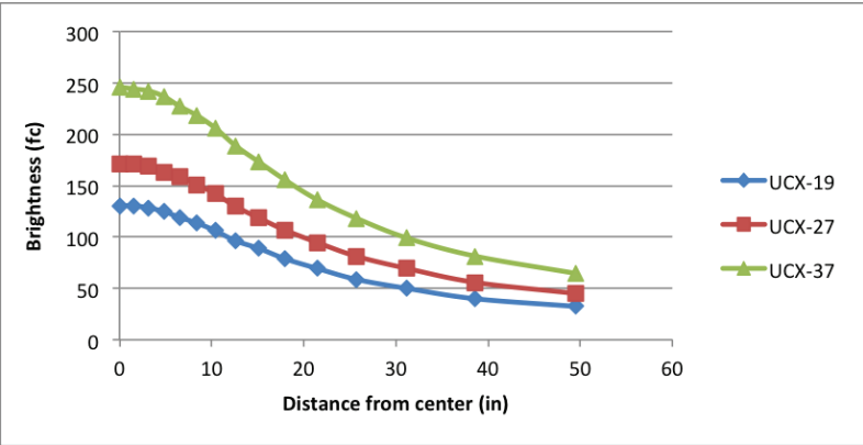
Photometrics: Light source placed 18" away from work surface. Graph represents 5,000 K light.
