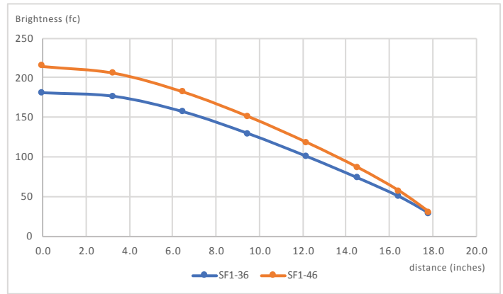
Photometrics: light source placed 19" away from work surface
