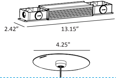
Remote Transformer
